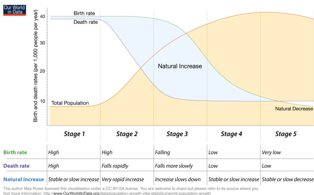
Figure 4. Demographic transition.
